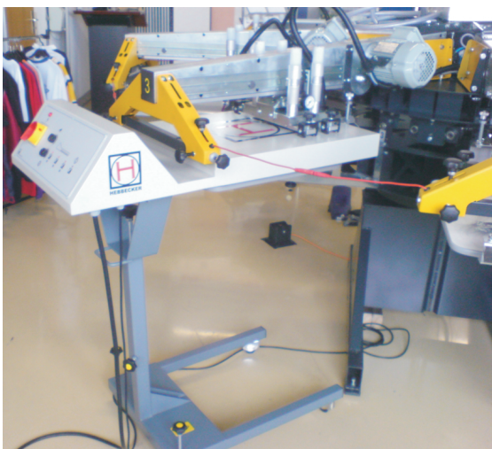
S-flash integrated in printingstation
